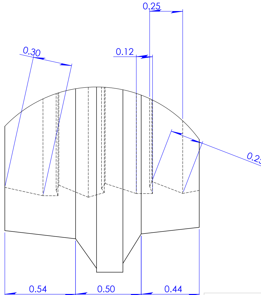
DETAIL A SCALE 2 : 0.75
